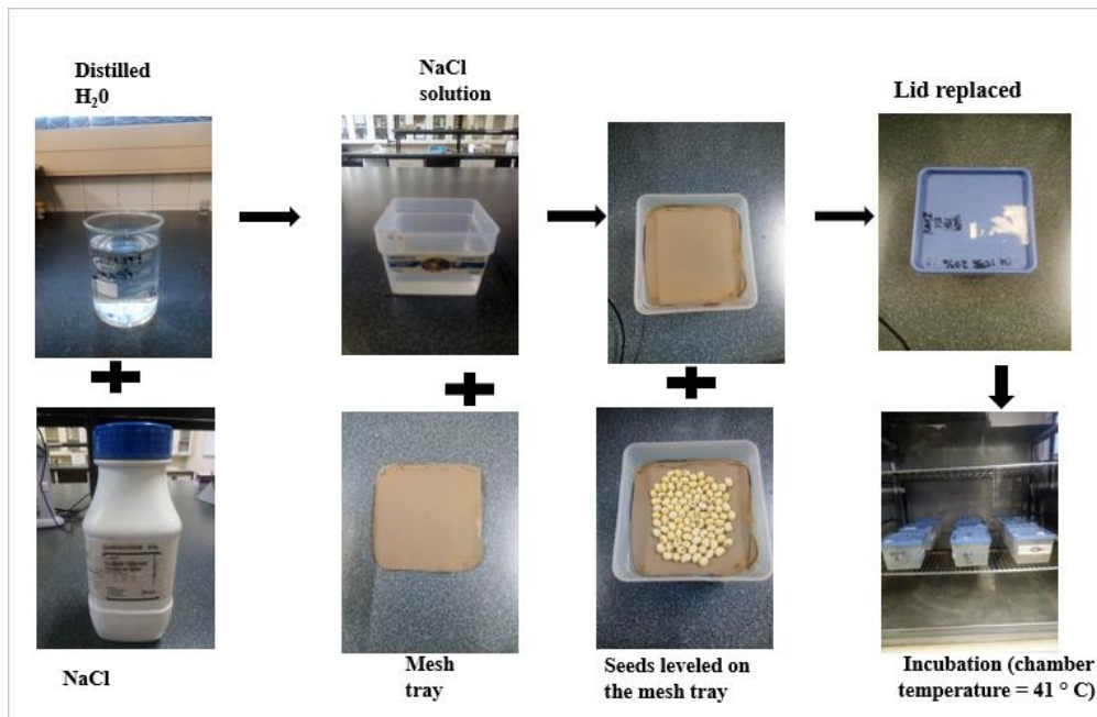
Figure 3.1 Schematic illustration for the accelerated aging experiment set-up.
