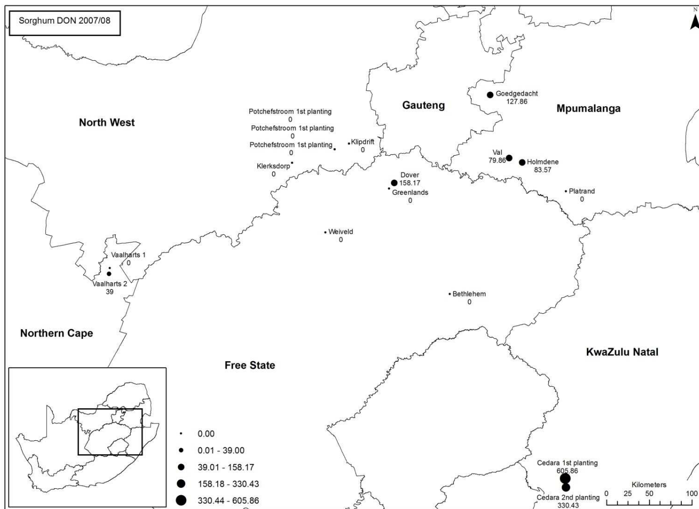
Figure 3.7. Distribution of DON ( \mu\text{g/kg} ) in sorghum grain samples collected during the 2007/08 season from different grain production areas of South Africa. The Jenks natural breaks classification method was used to arrange values into different classes.
