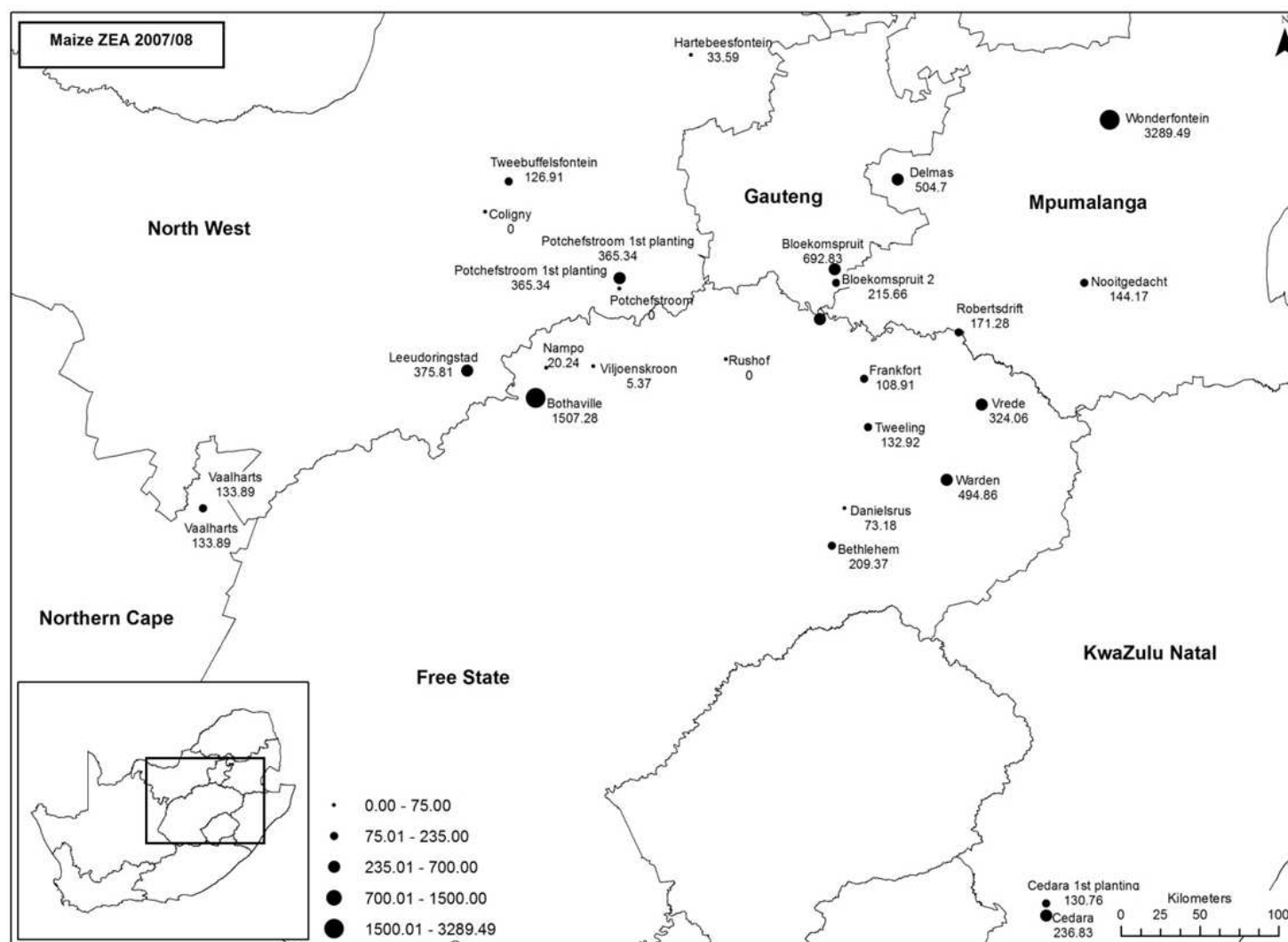
Figure 3.5. Distribution of ZEA ( \mu\text{g/kg} ) in maize kernel samples collected during the 2007/08 season from different grain production areas of South Africa. The Jenks natural breaks classification method was used to arrange values into different classes.
