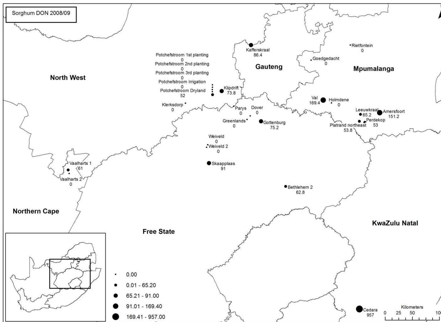
Figure 3.8. Distribution of DON ( \mu\text{g/kg} ) in sorghum grain samples collected during the 2008/09 season from different grain production areas of South Africa. The Jenks natural breaks classification method was used to arrange values into different classes.
