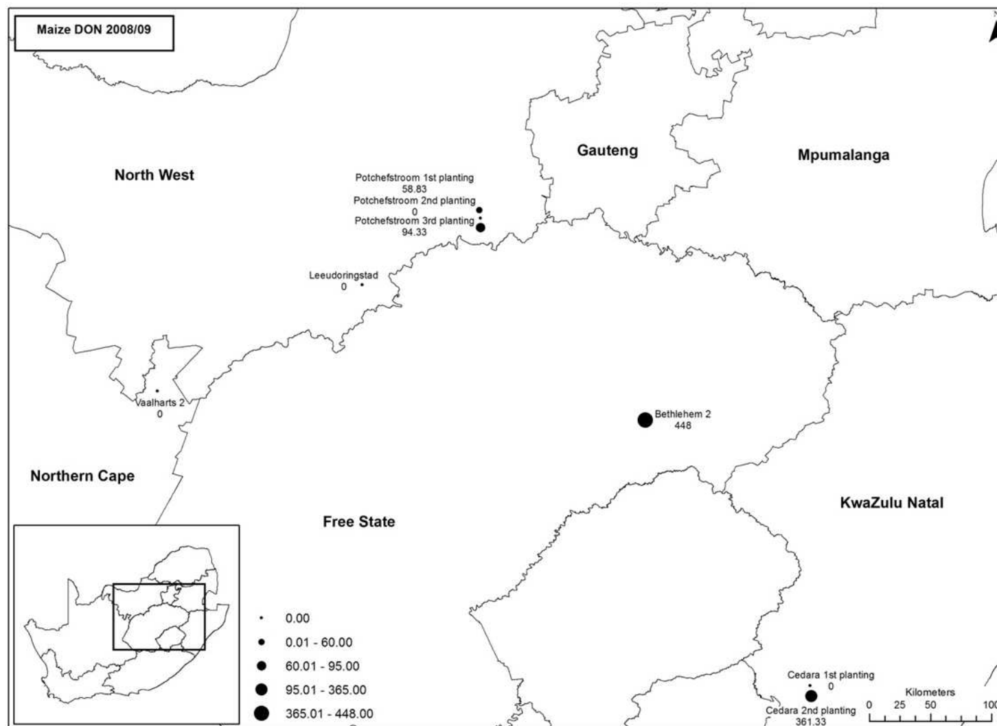
Figure 3.3. Distribution of DON ( \mu\text{g/kg} ) in maize kernel samples collected during the 2008/09 season from different grain production areas of South Africa. The Jenks natural breaks classification method was used to arrange values into different classes.
