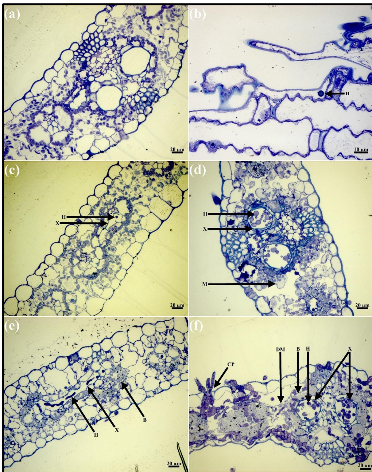
Figure 3.2. Light microscopy of B73 maize leaves during Exserohilum turcicum infection. (a) Uninoculated maize leaf showing a major vein with a minor vein in close proximity, intact spongy mesophyll cells, epidermis and bundle sheath cells are visible; (b) hyphal growth present in an epidermal cell (9 days post-inoculation, dpi); (c) hyphal growth present in a xylem vessel of one of the minor veins (11 dpi); (d) abundant hyphae present in the xylem vessel in
